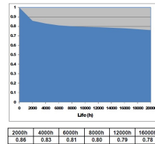
LUMEN MAINTENANCE
