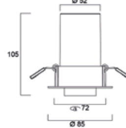
Retractable downlight
