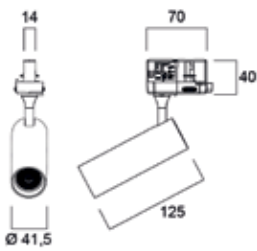
Tracklight
