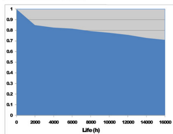
LUMEN MAINTENANCE
